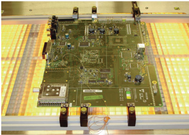
IR-4 Preheater
